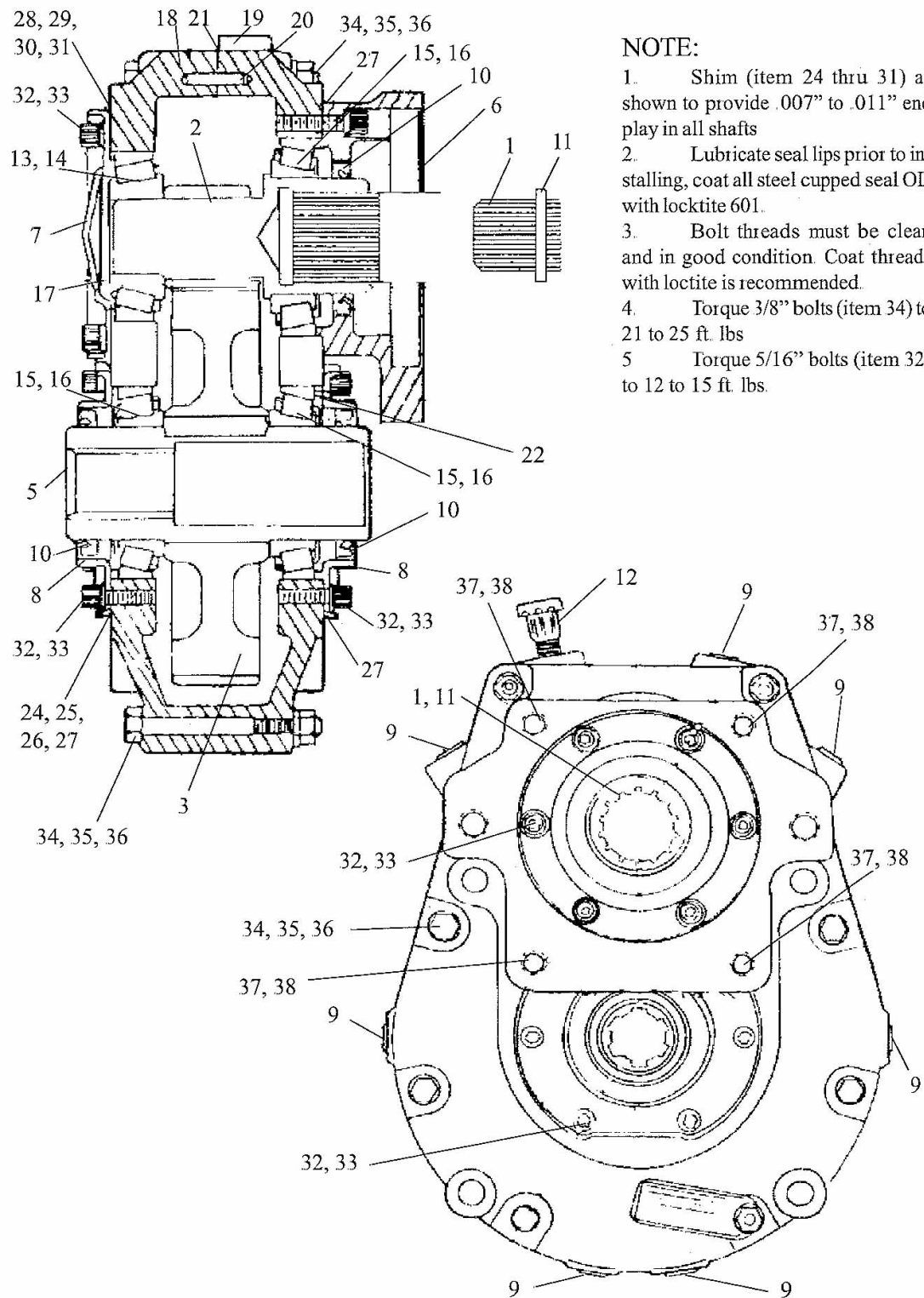
Speed Increaser Asy 540 rpm - P/N 00751488
