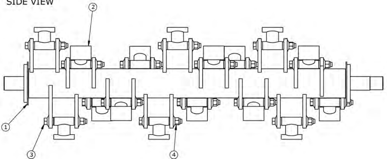
SIDE VIEW
