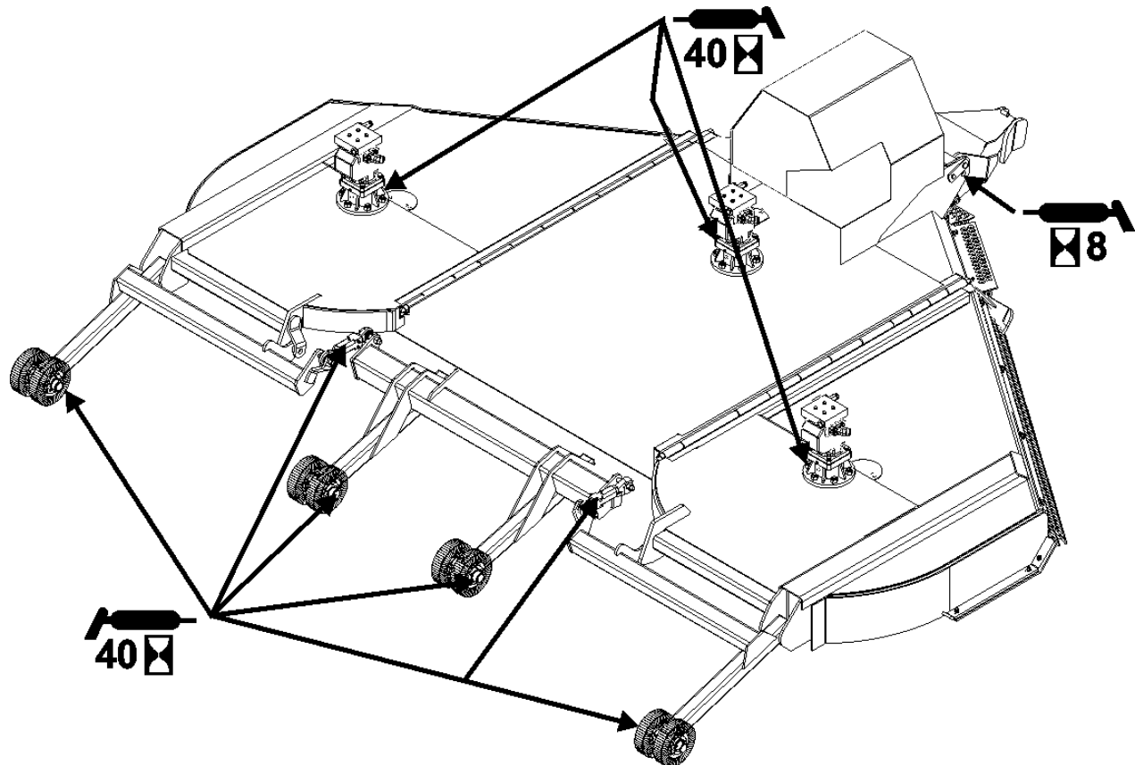
Lubrication/Fitting Location
